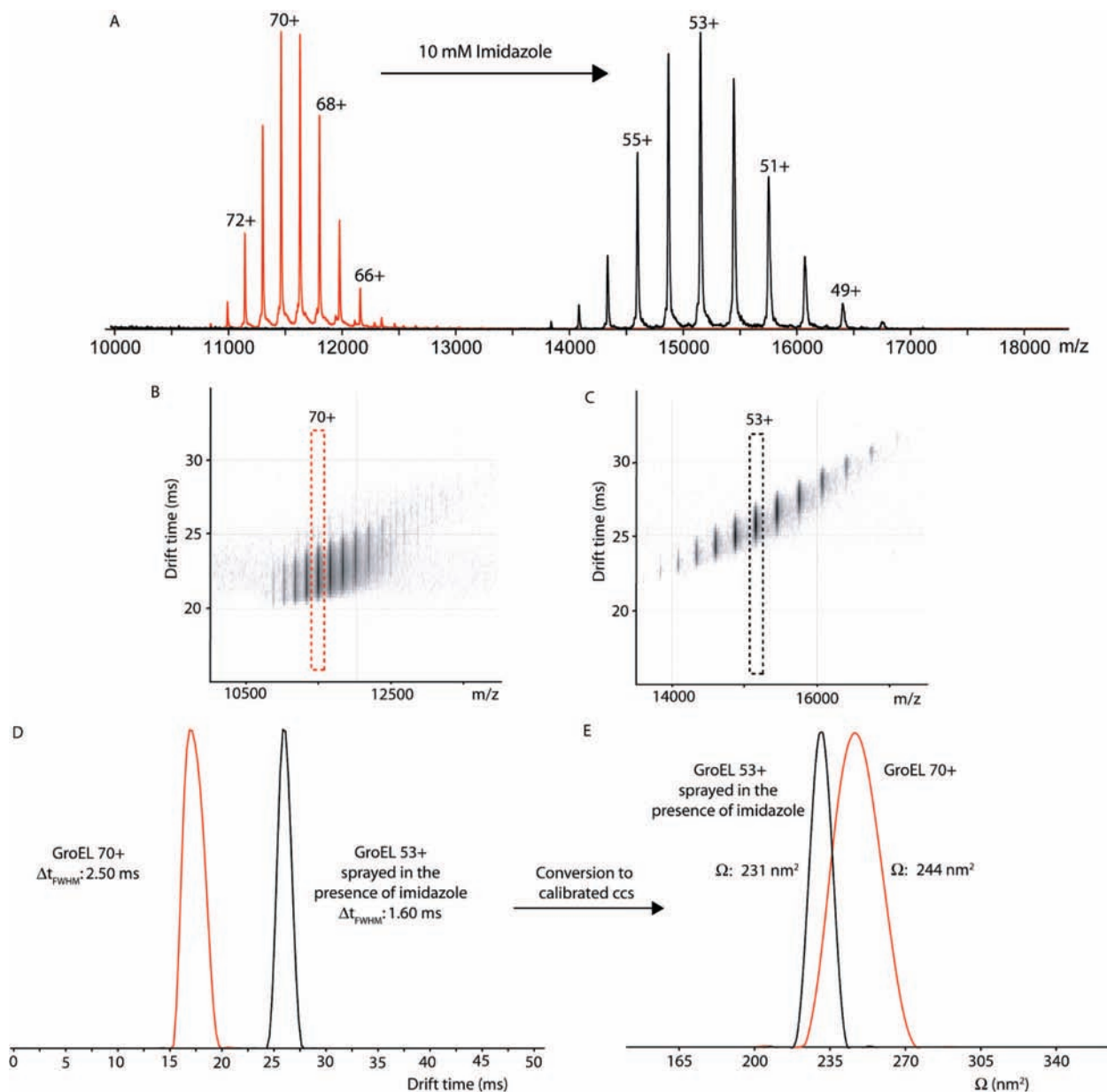
Figure 2. (A) Overlaid nano-ESI mass spectra of 5 \mu\text{M} GroEL sprayed from 50 mM ammonium acetate pH 6.9 (red) and 5 \mu\text{M} GroEL sprayed from 50 mM ammonium acetate pH 6.9 + 10 mM imidazole (black). The addition of imidazole significantly lowers the average charge state distribution of GroEL. (B) Corresponding uncorrected drift time profiles of GroEL and (C) GroEL sprayed in the presence of imidazole. The most intense charge states (boxed) were selected to create ccs distribution plots. (D) The 70+ GroEL ion peak has a resolution of 7 ( R = t_p/\Delta t_{\text{whm}} ), and the 53+ GroEL ion peak has a resolution of 17. Averaging over all charge states, the resolution increases from 7 to 18 for GroEL after the addition of imidazole to the spray solution. (E) Conversion of the absolute drift time into a calibrated ccs clearly shows the narrowing of the ccs distribution for GroEL ions due to the addition of imidazole to the ESI spray solution.
